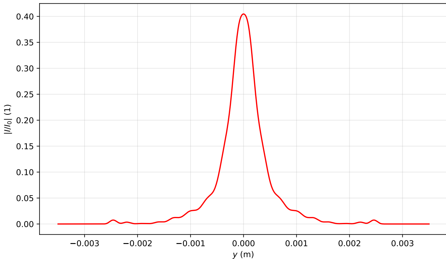
Intensity profile I(x=0, y, z=1.911)/I_0 , \text{Pin}=3.0\text{Pcr} , artificial time
